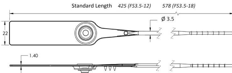
Fast Seal 3.5 Non Tear-Off (FS3.5 NTO)
